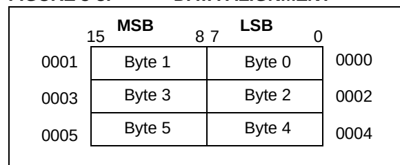
FIGURE 3-8: DATA ALIGNMENT
